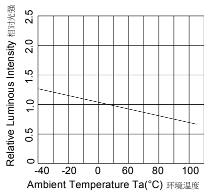
Ambient Temperature VS. Relative Intensity Ta-IV曲线
